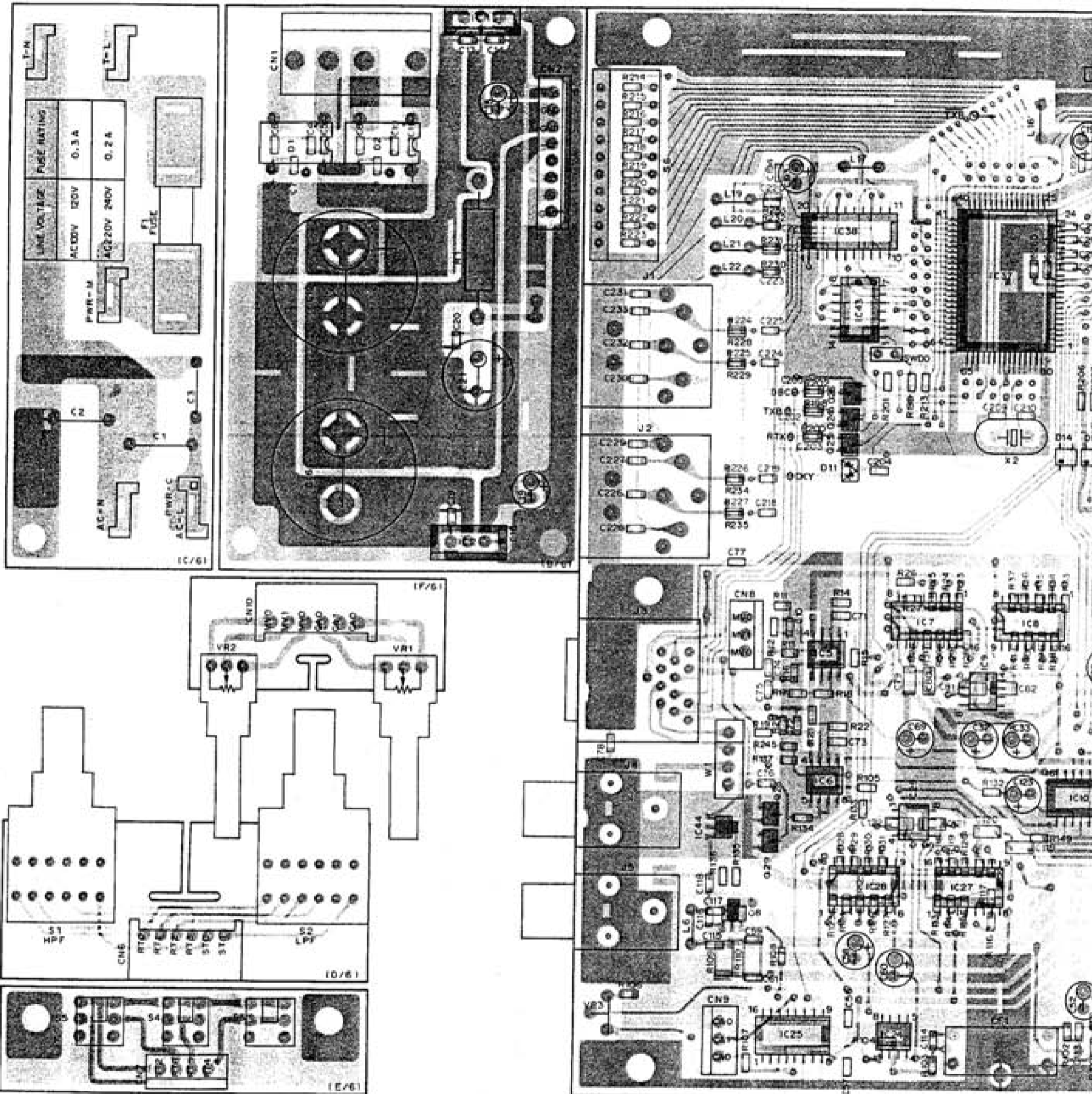
DSP UNIT (X53-3360-00) Component side view
