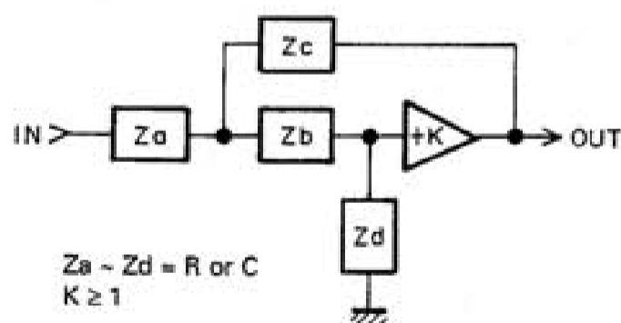
(a) Analog filter (active filter)
