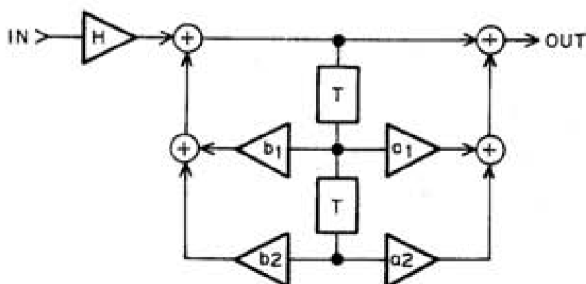
(b) Digital filter
